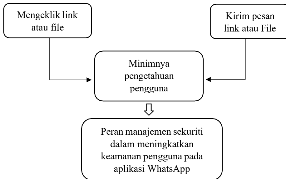
Gambar 1. Conceptual Framework
